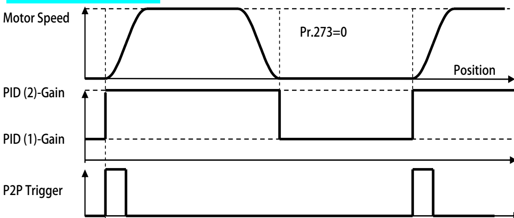
BP2P PID When Lock Time = 0
