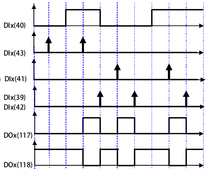
Truth Table:(D Type Flip/Flop)
