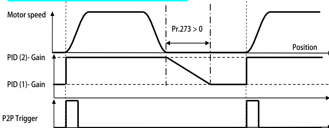
BP2P PID When Lock Time > 0 & P2P Trigger When Finished
